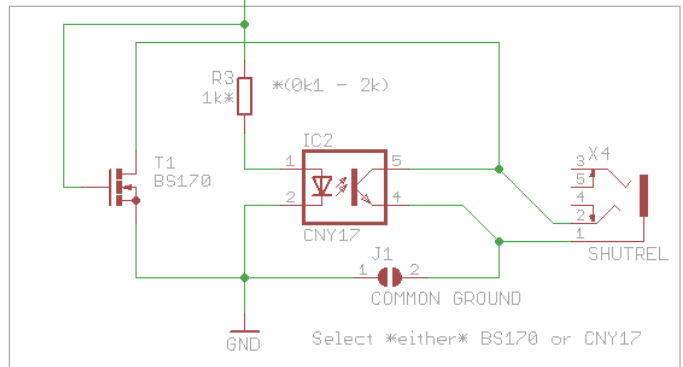
Shutter release
